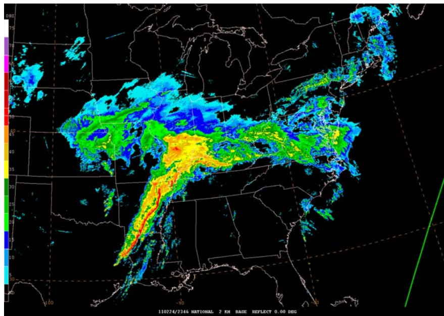
Figure 8: Mosaic reflectivity image from 2346 UTC on 24 February, 2011.
