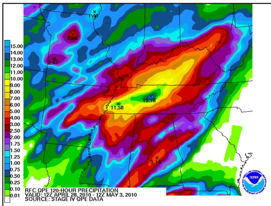
Figure 2: Total rainfall from 12 UTC on 28 April through 12 UTC on 3 May, 2010.
