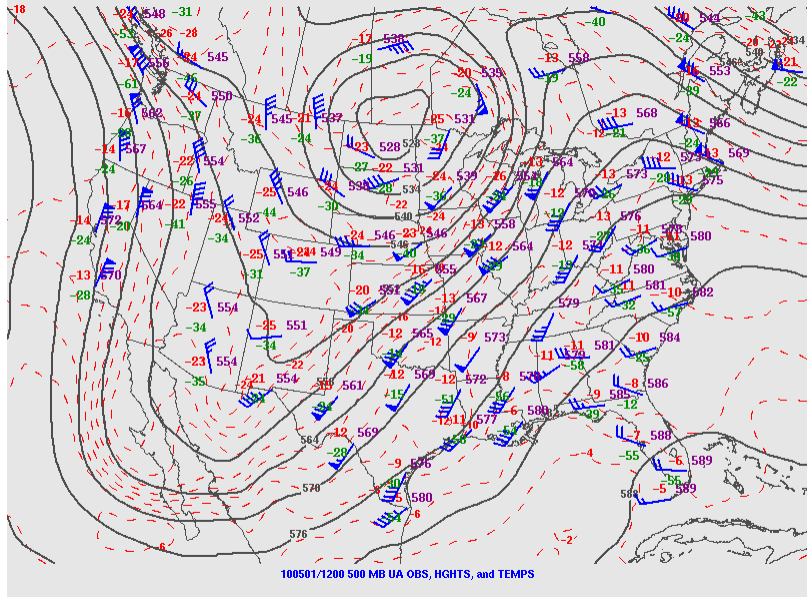
Figure 4: 500 hPa analysis from 12 UTC on 1 May, 2010 (SPC).
