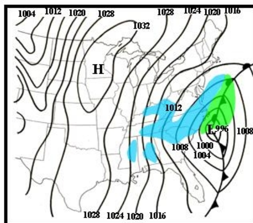
1200 UTC 26 December 2010
