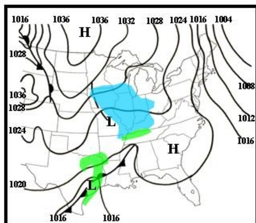
0000 UTC 25 December 2010
