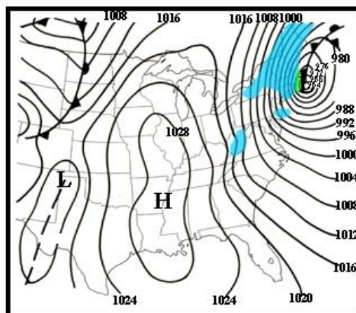
1200 UTC 27 December 2010
