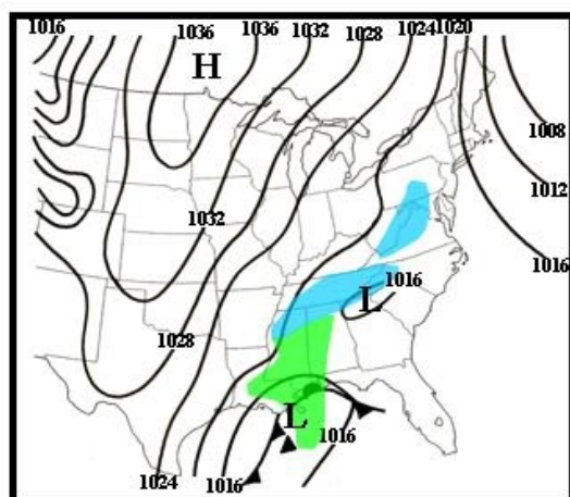
1200 UTC 25 December 2010
