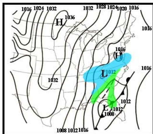
0000 UTC 26 December 2010
