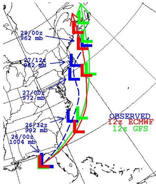
Fig. 18. Comparison of observed cyclone track to the operational 1200 UTC 23 December ECMWF and GFS forecasts.
