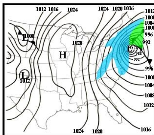
0000 UTC 27 December 2010
