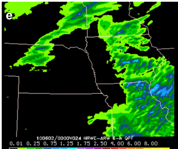
Figure 3. (a) NSSL Q2 QPE for the 6 hr period ending 0000 UTC 2 June 2010 and the corresponding 6 hr precipitation forecasts from the (b) NAM, (c) WRF-NSSL4, (d) WRF-NMM4, and (e) HRWE-ARW initialized at 0000 UTC 1 June 2010.
