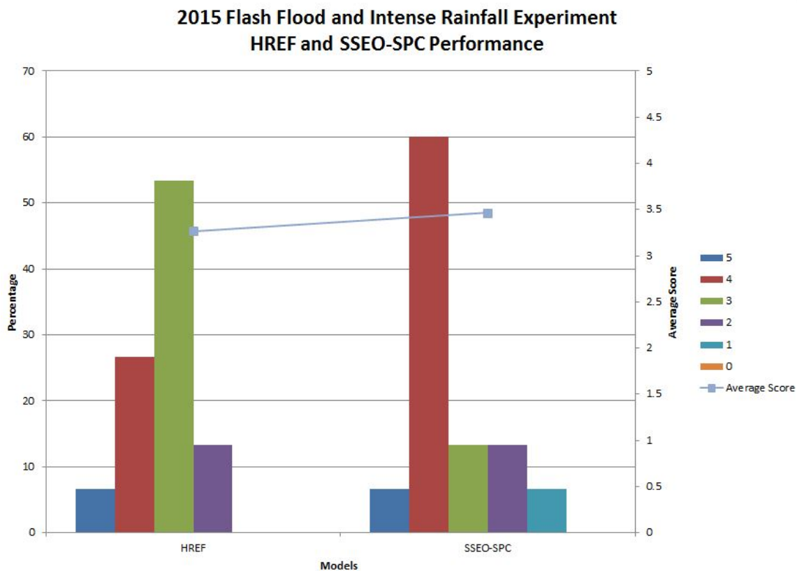
Figure 11 Experimental ensemble model performance based on feedback from subjective model evaluations conducted during the 2015 Flash Flood and Intense Rainfall Experiment. Participants were asked to rate the performance of each model on a scale of 1 ( very poor ) to 5 ( very good ). The Average Score is a numerical average of all scores calculated over the experiment, not an average of the percentages shown.
