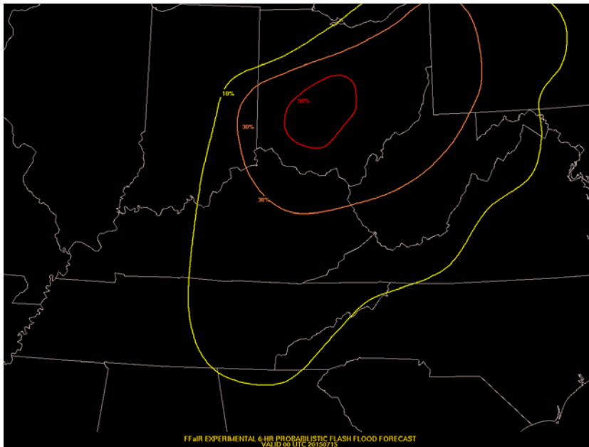
Figure 3. Experimental probability of flash flooding forecast graphic valid from 18Z on July 14, 2015 to 00Z on July 15, 2015. 10% probabilistic contours are in yellow, 30% in orange, and 50% in red.
