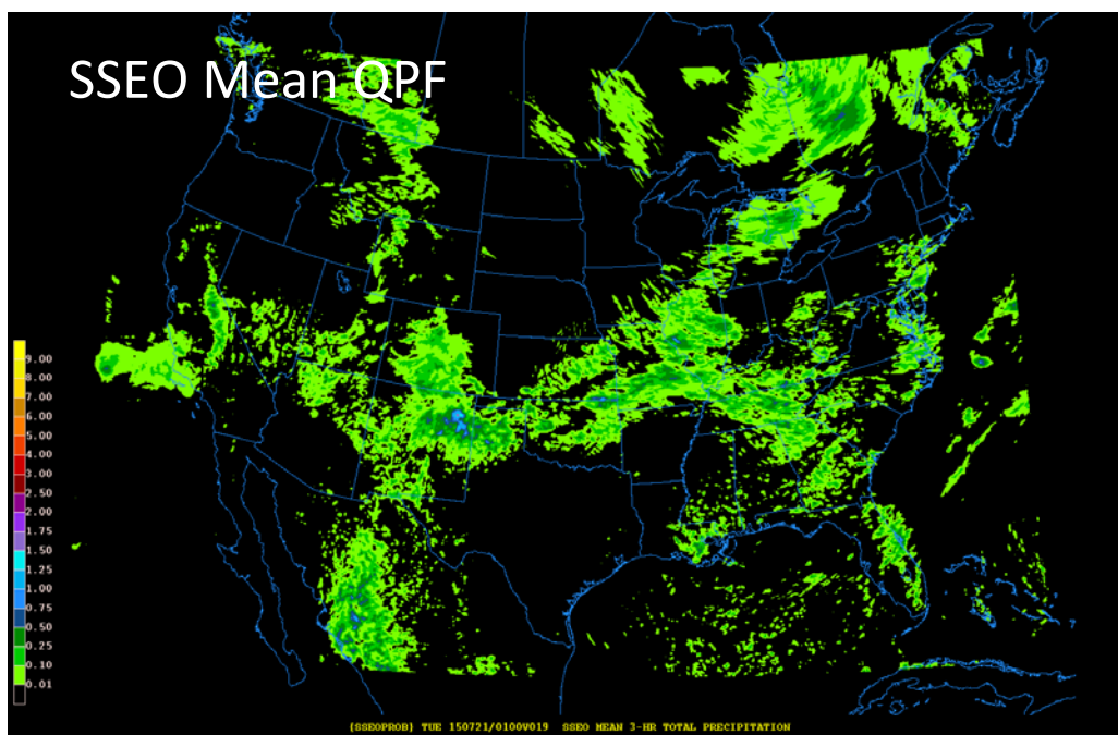
Figure 12. The SSEO forecast for 3-hour mean QPF on July 15, 2015.
