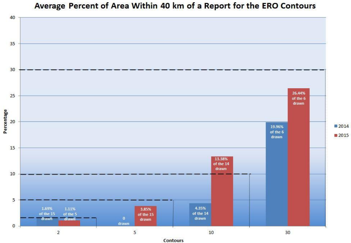
Figure 21. A comparison of the average percent of area of the ERO contours drawn from the 2014 (blue) and 2015 (red) experiments falling within 40 km of a reported observation of flooding or flash flooding. The horizontal dashed lines indicate the percent of each contour and the value the forecasts should equal if they showed perfect skill/calibration. Note that the 5% contour was not available during the 2014 FFaIR Experiment.
