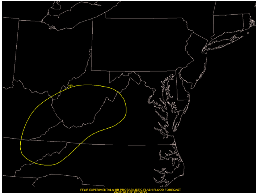
Figure 5. Experimental probability of flash flooding forecast graphic valid 00- 06 UTC on July 15, 2015
