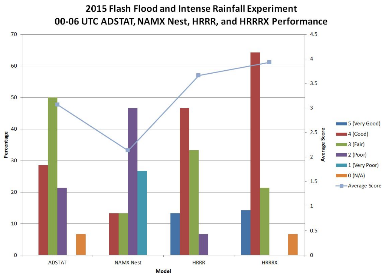
Figure 8. Experimental deterministic model performance based on feedback from subjective model evaluations conducted during the 2015 Flash Flood and Intense Rainfall Experiment. Participants were asked to rate the performance of each model on a scale of 1 (very poor) to 5 (very good). The Average Score is a numerical average of all scores calculated over the experiment, not an average of the percentages shown.
