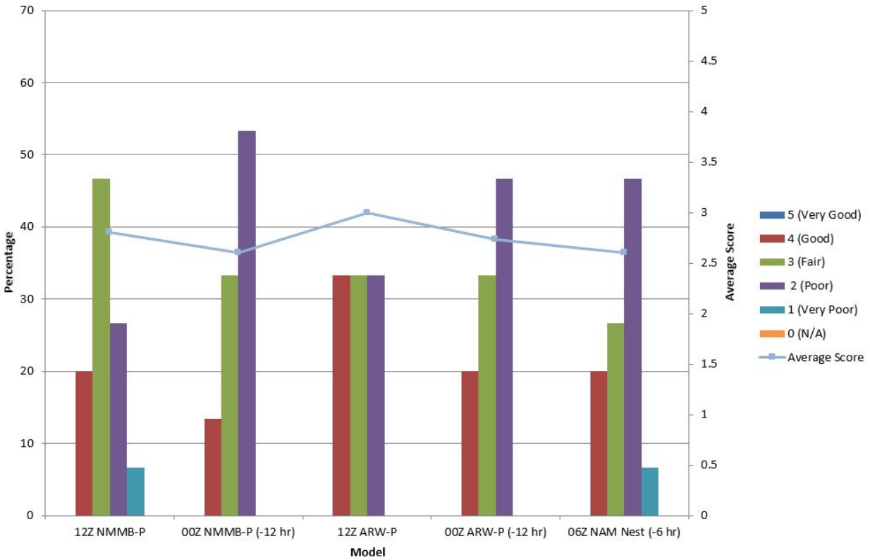
Figure 17. Time-lagged member performance based on feedback from subjective model evaluations conducted during the 2015 Flash Flood and Intense Rainfall Experiment. Participants were asked to rate the performance of each model on a scale of 1 (very poor) to 5 (very good). The Average Score is a numerical average of all scores calculated over the experiment, not an average of the percentages shown.
