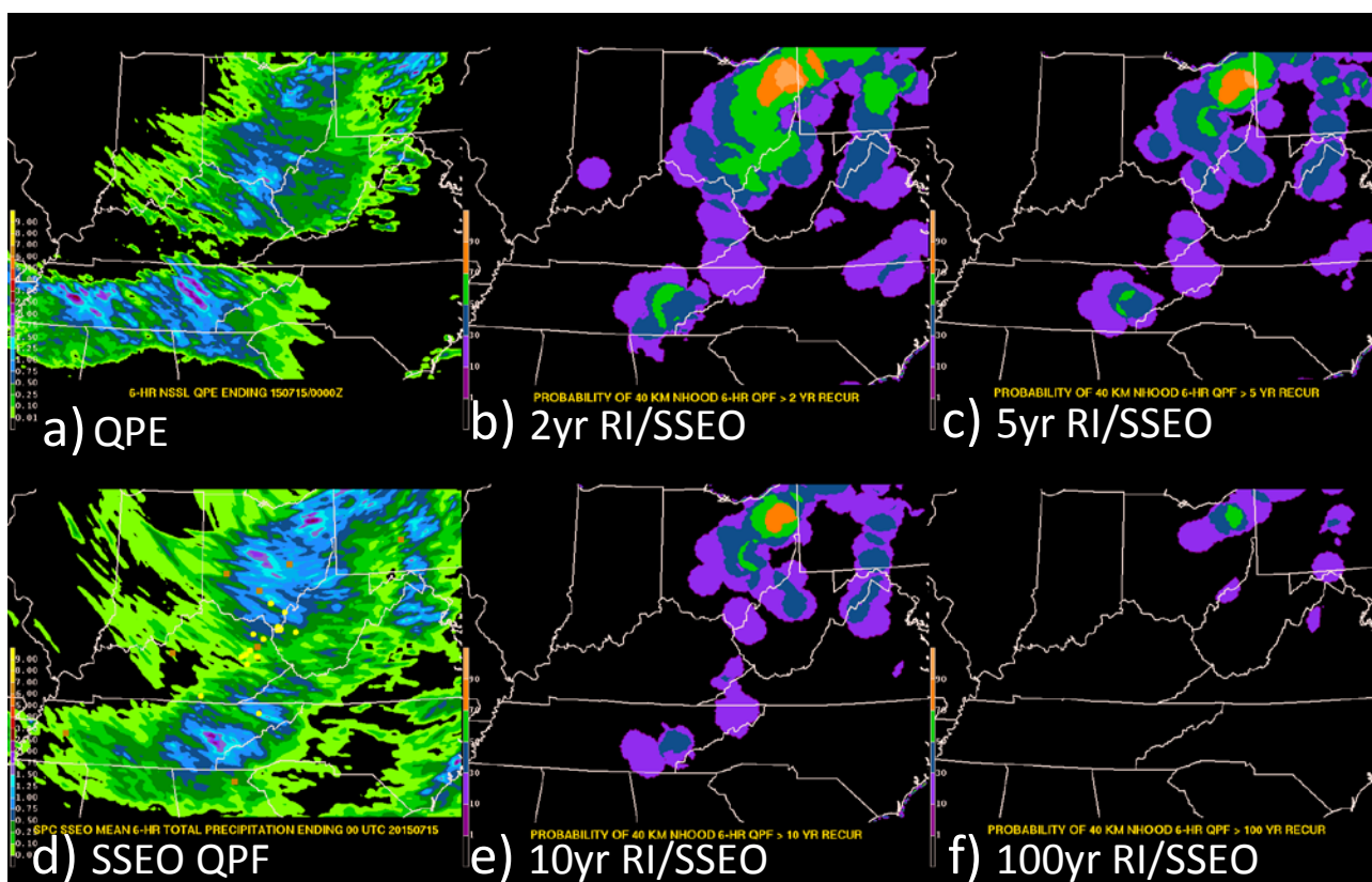
Figure 15. FFaIR Participants used this display to subjectively rank the value of the Recurrence Intervals. (a) NSSL 6-hr QPE, (b) 2-year Recurrence Intervals as derived by the SSEO 6-hr mean QPF, (c) 5-year Recurrence Interval, (d) SSEO 6-hr mean QPF and flash flooding reports, (e) 10-year Recurrence Interval, (f) 100-year Recurrence Interval.
