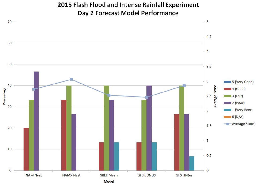
Figure 16. Model evaluation for creating a Day 2 Excessive Rainfall forecast based on feedback from subjective feedback collected during the 2015 Flash Flood and Intense Rainfall Experiment. Participants were asked to rate the performance of each model on a scale of 1 (very poor) to 5 (very good). The Average Score is a numerical average of all scores calculated over the experiment, not an average of the percentages shown.
