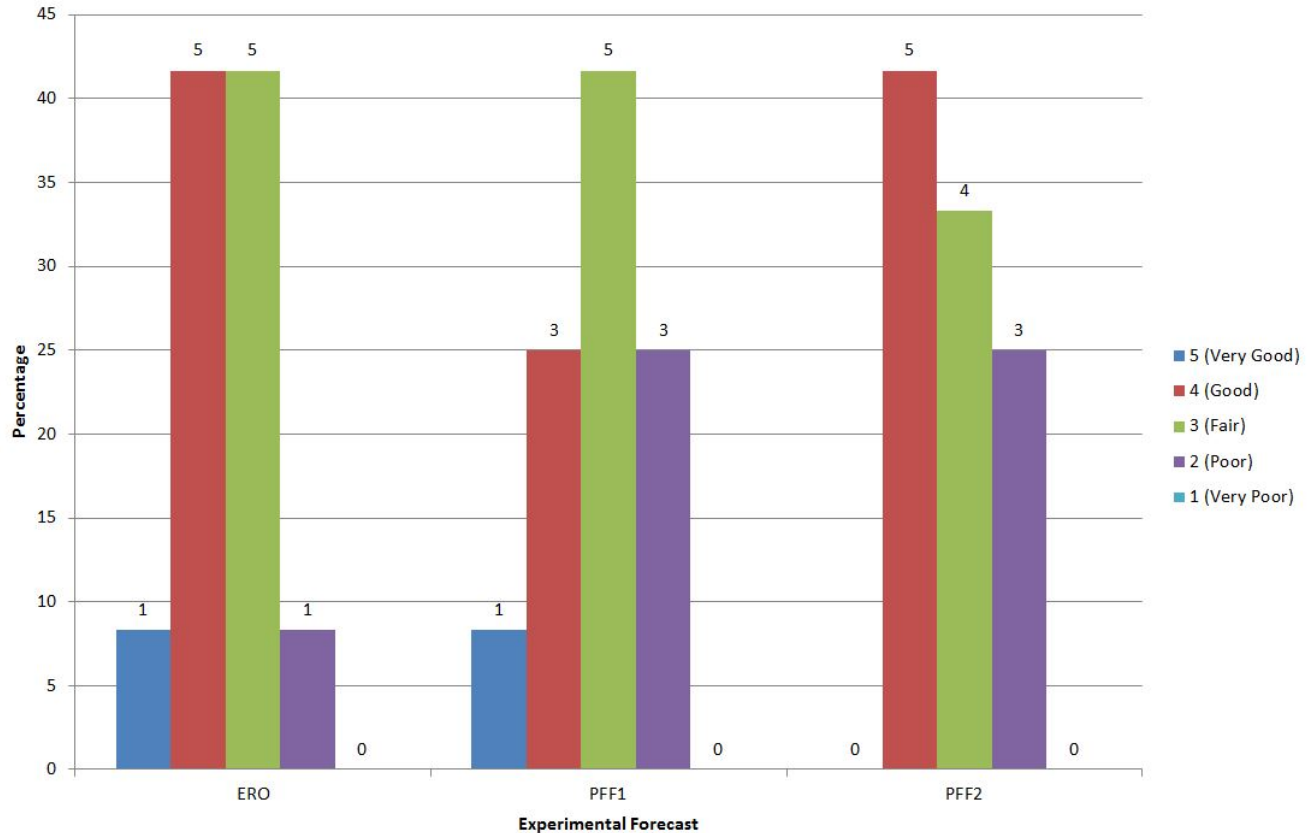
Figure 20. The rating for each of the three experimental forecasts completed in FFaIR: the 15-12 UTC probabilistic excessive rainfall outlook (ERO), the 18-00 UTC probabilistic flash flood forecast (PFF1) and the 00-06 UTC probabilistic flash flood outlook (PFF2).
