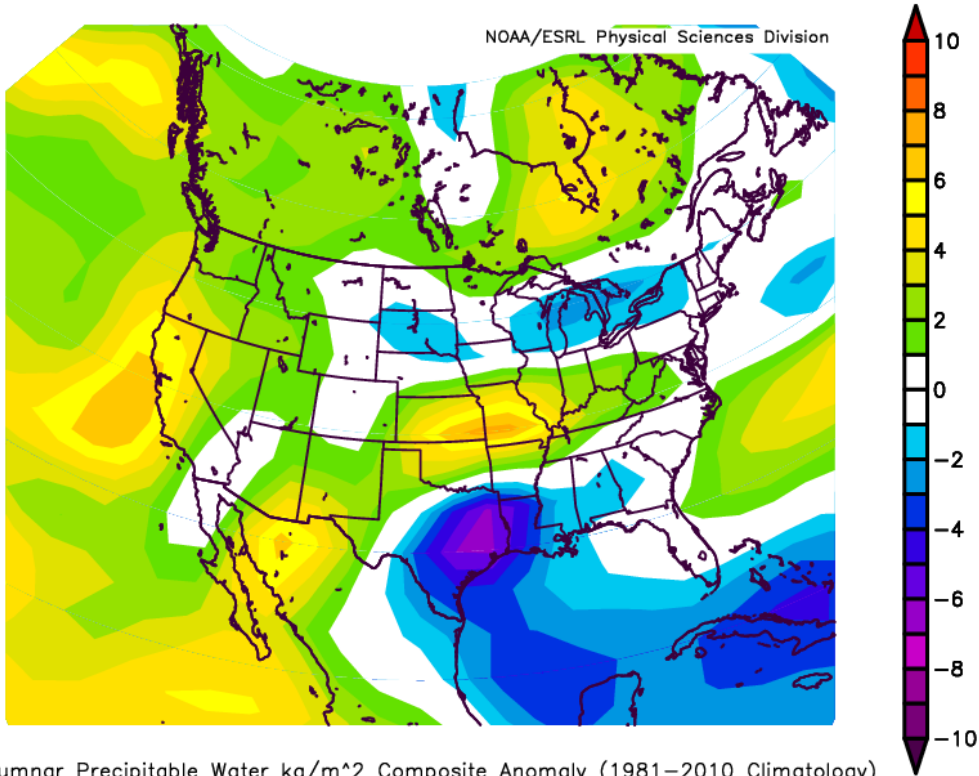
Columnar Precipitable Water \text{kg/m}^2 Composite Anomaly (1981–2010 Climatology) 7/6/15 to 7/24/15 NCEP/NCAR Reanalysis
