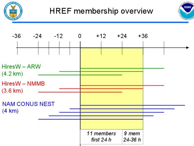
Figure 1. Membership overview of the HREF Ensemble from EMC.
