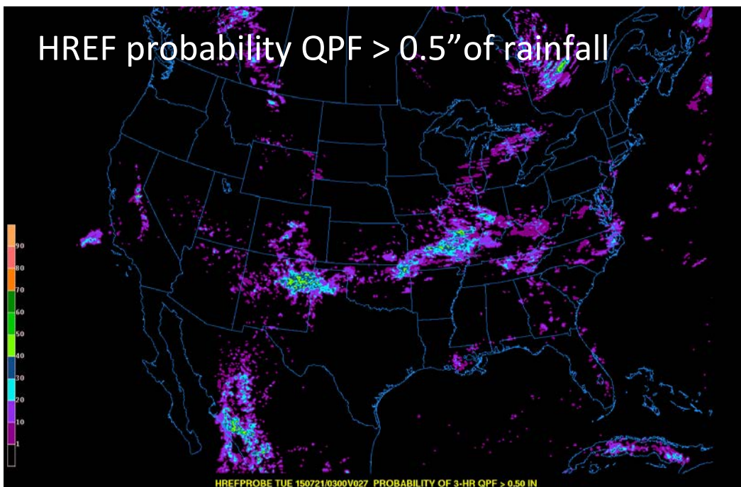
Figure 14. The HREF probability of the same 3-hour mean QPF being greater than 0.5 inches of rainfall on July 15, 2015.
