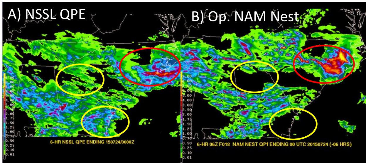
Figure 18. A) An example of the NSSL QPE the B) time-lagged 4 km operational NAM Nest and during the 2015 FFaIR Experiment. The red oval indicates an area in which the NAM Nest the maximum QPF was too intense. The yellow ovals indicate lighter precipitation areas in which the NAM Nest was too light or non-existent.
