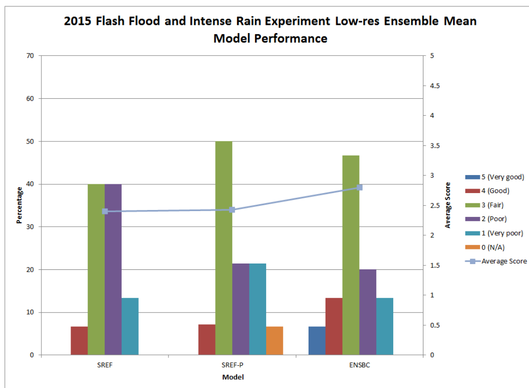
Figure 10. Operational and experimental low-resolution ensemble model performance based on feedback from subjective model evaluations conducted during the 2015 Flash Flood and Intense Rainfall Experiment. Participants were asked to rate the performance of each model on a scale of 1 (very poor) to 5 (very good). The Average Score is a numerical average of all scores calculated over the experiment, not an average of the percentages shown.
