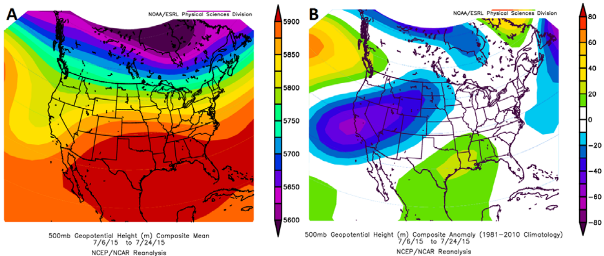
Figure 6. A) Composite mean 500 hPa geopotential heights over the three week experiment period from July 6-July 24, 2015. B) Mean 500 hPa geopotential height anomalies over the same time period. Images generated from the NCEP/NCAR Reanalysis provided by NOAA/ESRL/Physical Sciences Division ( http://www.esrl.noaa.gov/psd/data/composites/day/ ).
