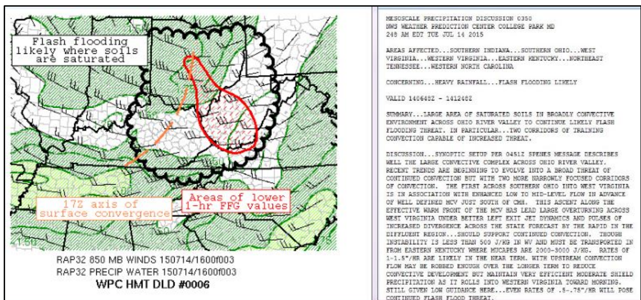
Figure 4. The 18-00 UTC Domain Limiting Discussion valid July 14, 2015.
